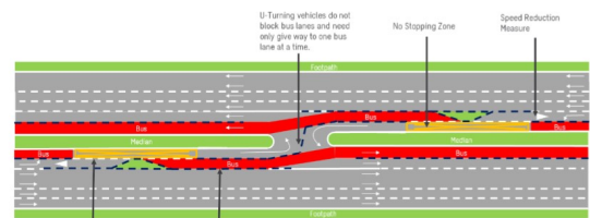
Figure 27 - Recommended U-Turn Proposal
